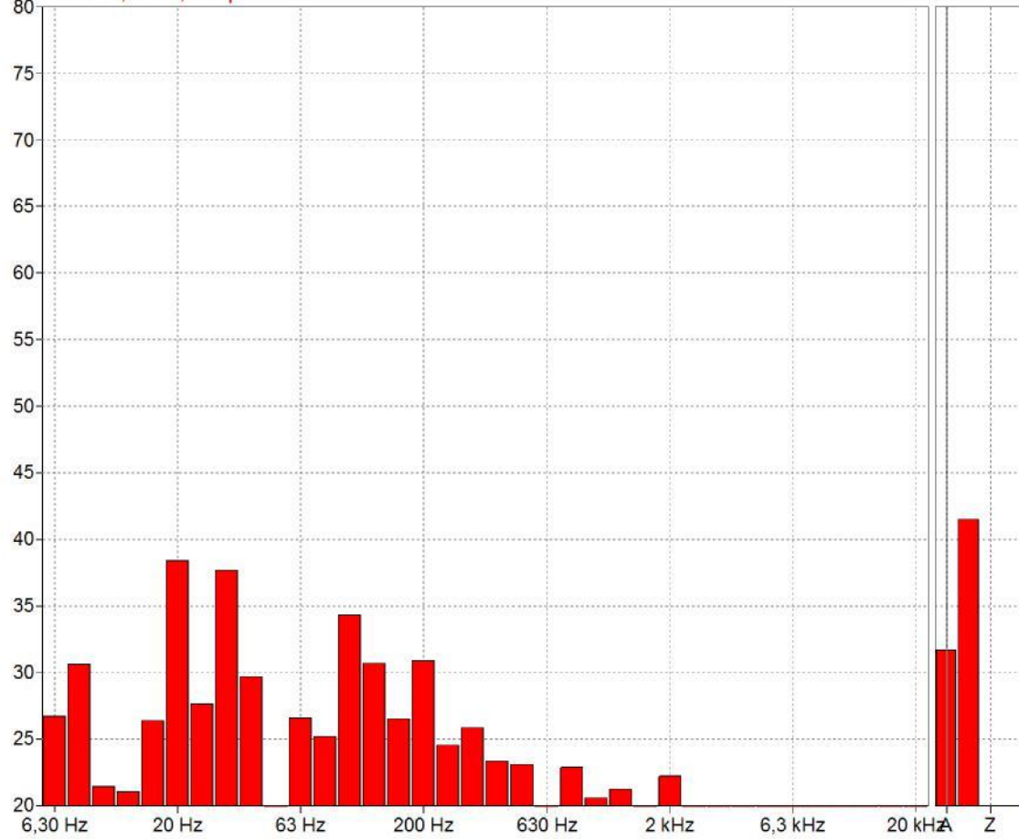
dB Profile, Ch1, Leq
